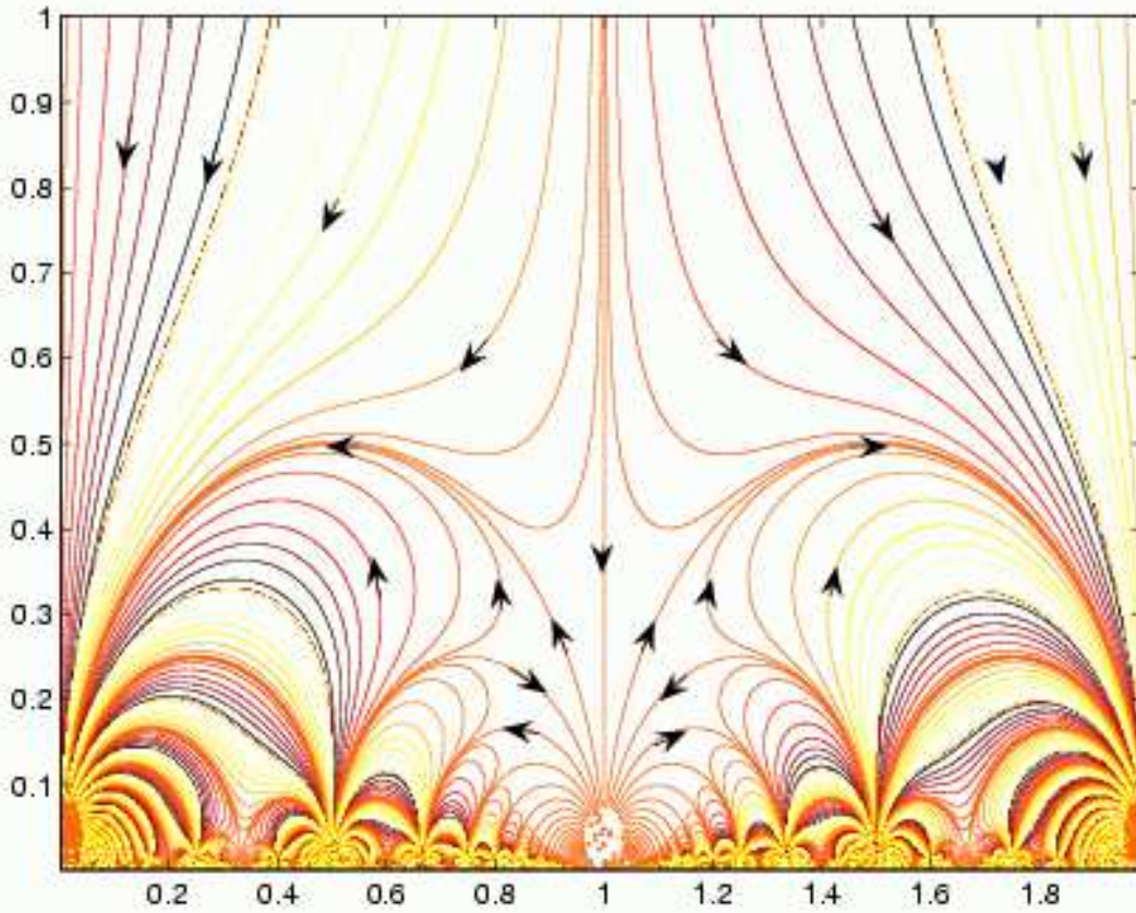
Fig. 1: Flow of effective coupling of N = 2 SUSY Yang-Mills, as the Higgs VEV is reduced, using (7). The pattern repeats under \tau \rightarrow \tau + 2 . There is a singularity at \tau = 1 and its images under \Gamma(2) . Note that \theta is driven to zero at strong coupling for any starting value between -2\pi and 2\pi at weak coupling.
